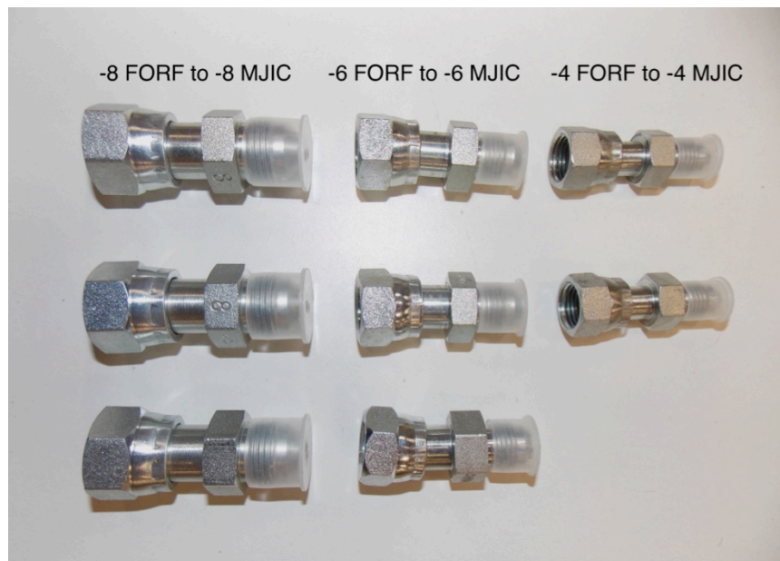
Figure 1: Hydraulic fitting sizes and quantities
