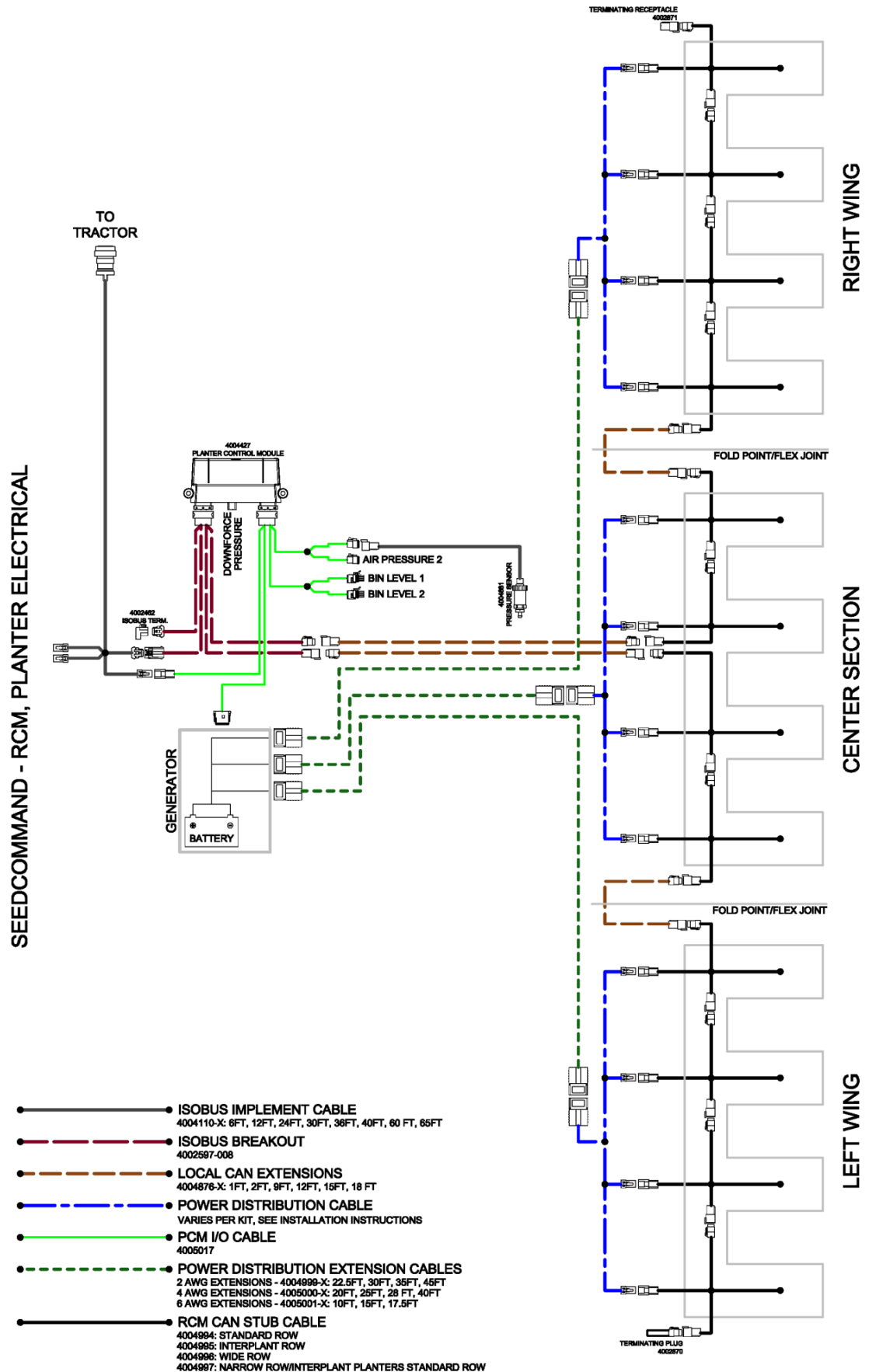
Figure 1: Cable Routing Diagram
